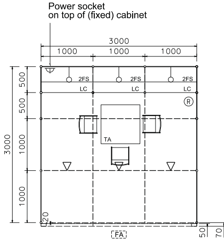
LAYOUT PLAN
