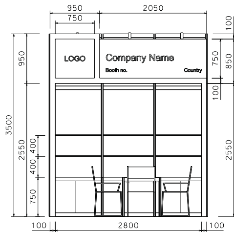
FRONT ELEVATION
