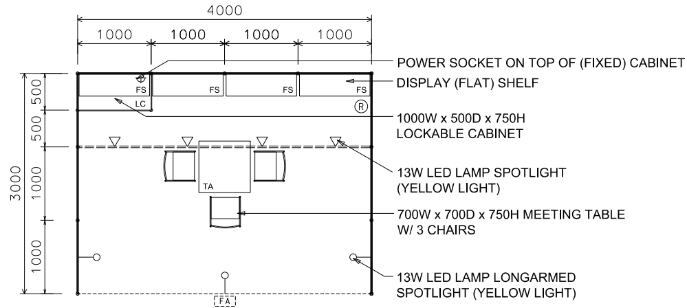
LAYOUT PLAN
