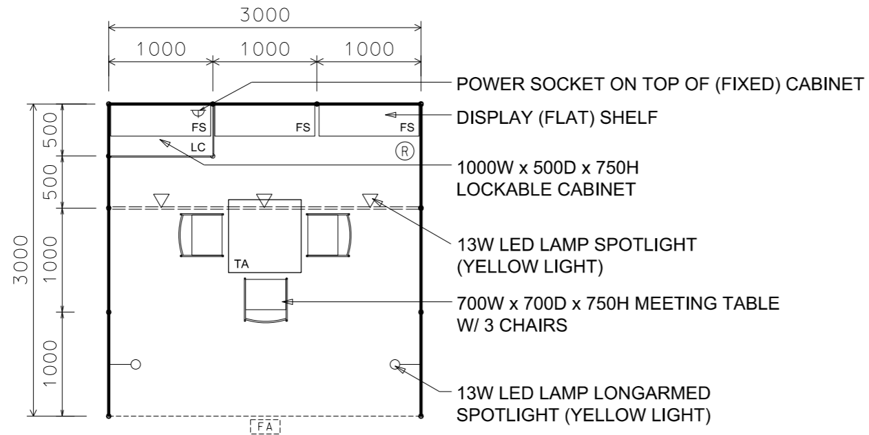
LAYOUT PLAN
